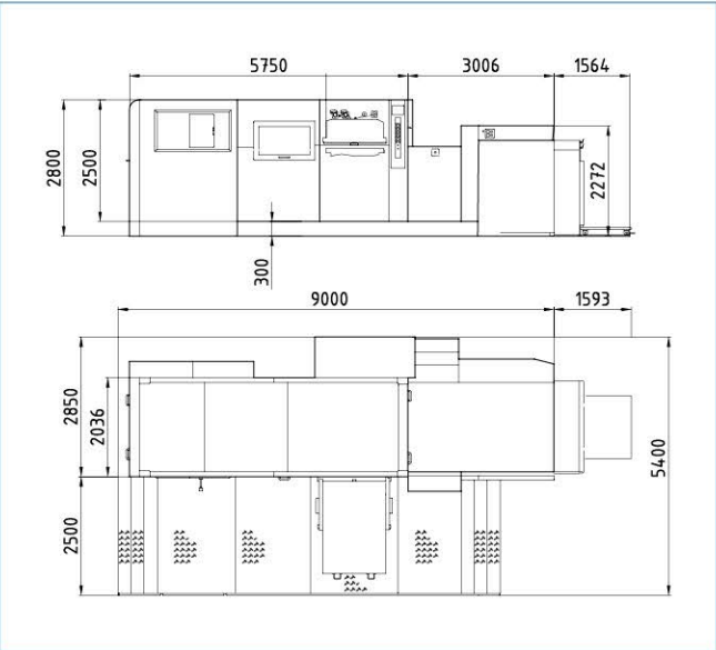
JY-1450 Floor Plan
