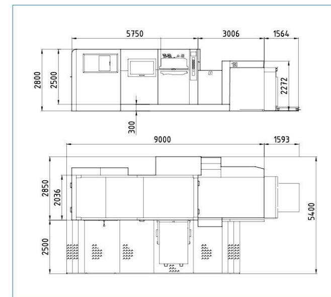
JY-1450 Floor Plan
