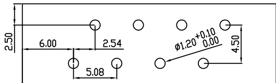
PCB Layout
