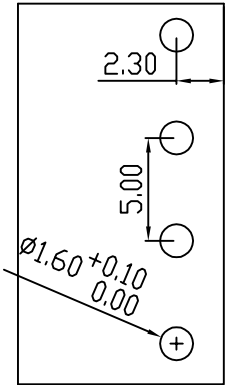
PCB LAYOUT
