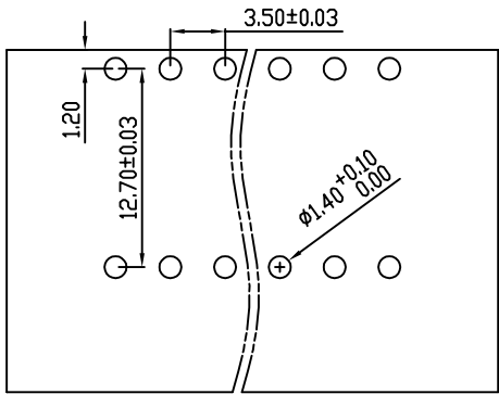
PCB LAYOUT
