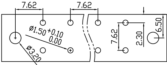
PCB LAYOUT
