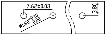
PCB LAYOUT
