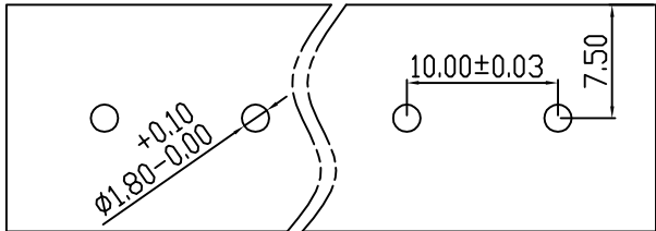
PCB LAYOUT
